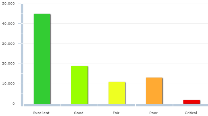
Wastewater Mains and Laterals Condition by Length (m)
