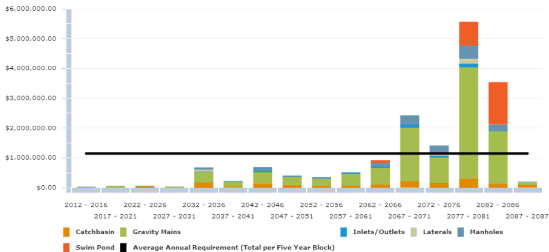
Storm Water Main Replacement Profile
